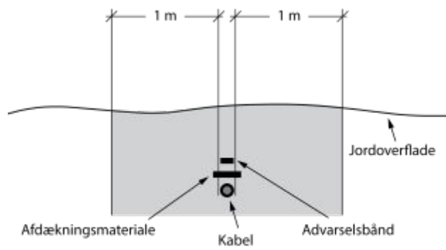
Figur 5 Kabler i jord
